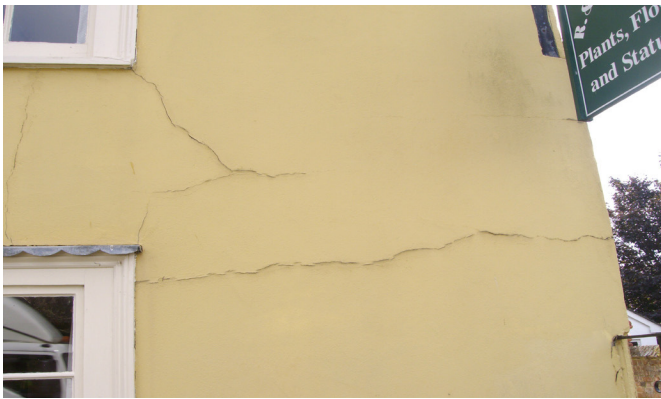
Figure 15: Hairline cracks resulting from the inappropriate use of cement render on traditionally constructed buildings can admit moisture via capillary action. Photo: Douglas Kent
